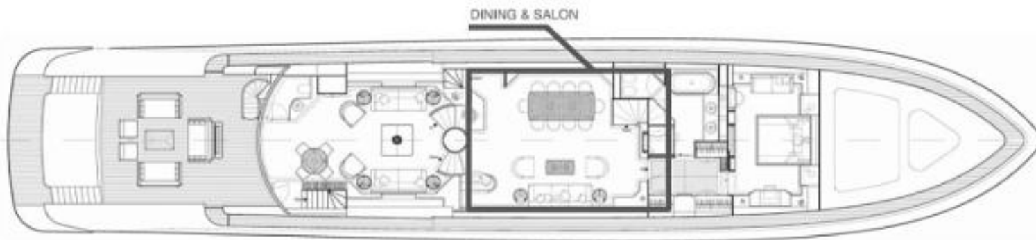
MAIN DECK
